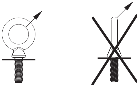
Figure 4.5: Fully seated eyebolts with washers, with correct orientation in the plane of pull (Correct; left, Incorrect; right)
